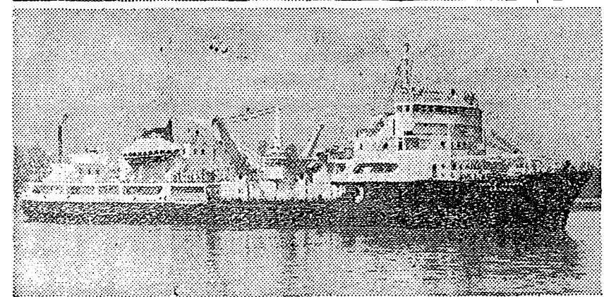
Left: Newest, largest, fastest sea-going hopper dredge on Great Lakes. With three times the capacity of any other, it can dredge to 43½-foot depth. Above: U. S. Markham's aft emergency station—emergency steering, magnetic and gyro compasses protected by fitted covers of Wellington Sears duck.
